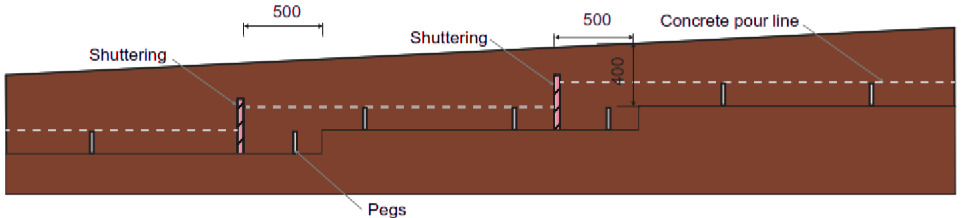
5.17 - Section through stepped foundation
