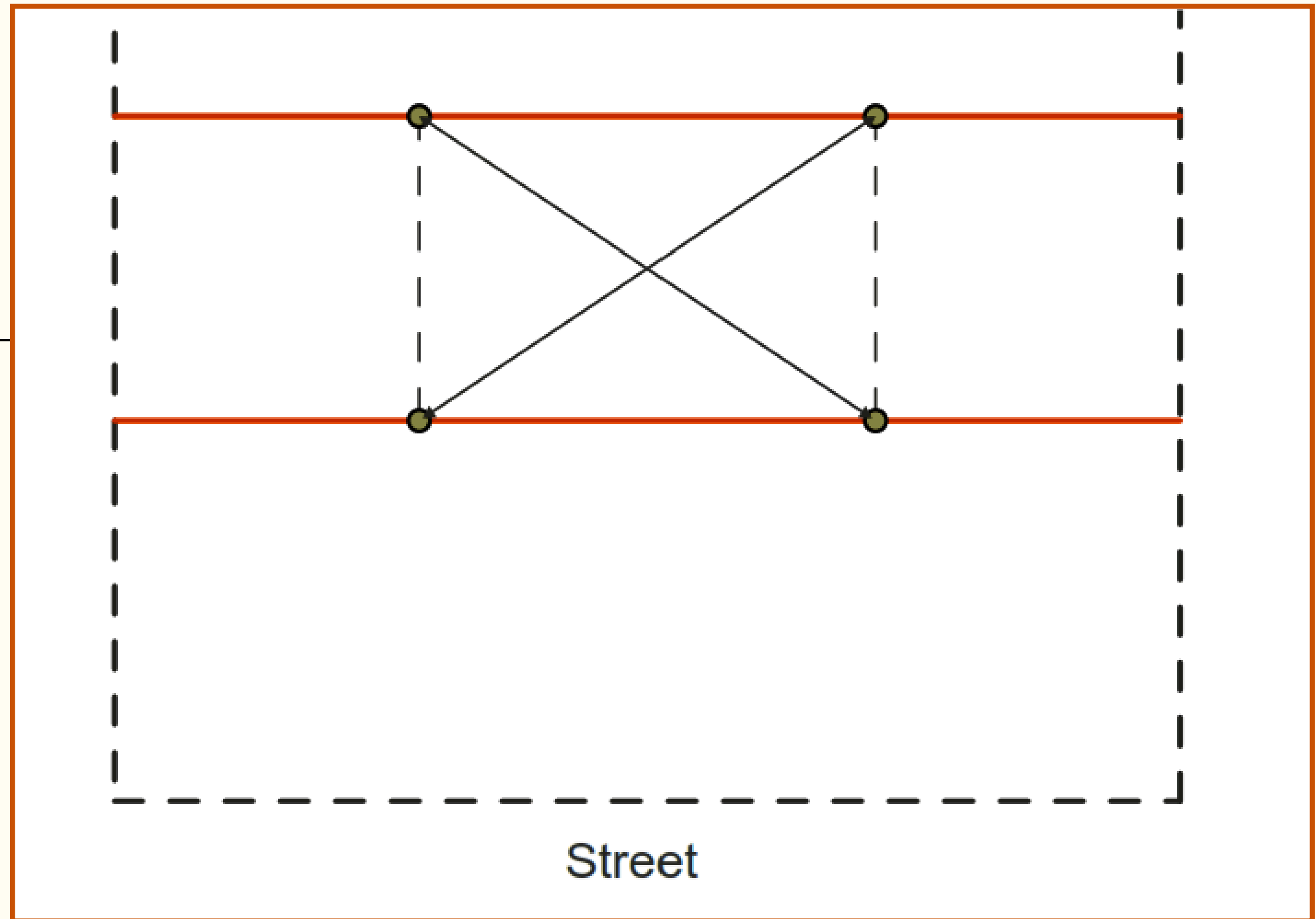
5.3 - This picture illustrates the four corner pegs established and with the profiles in position.
